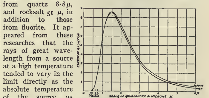
FIG. 8.—Distribution of energy in the spectrum of full radiation at 2000° Abs. according to formulae of Planck & Wien.
